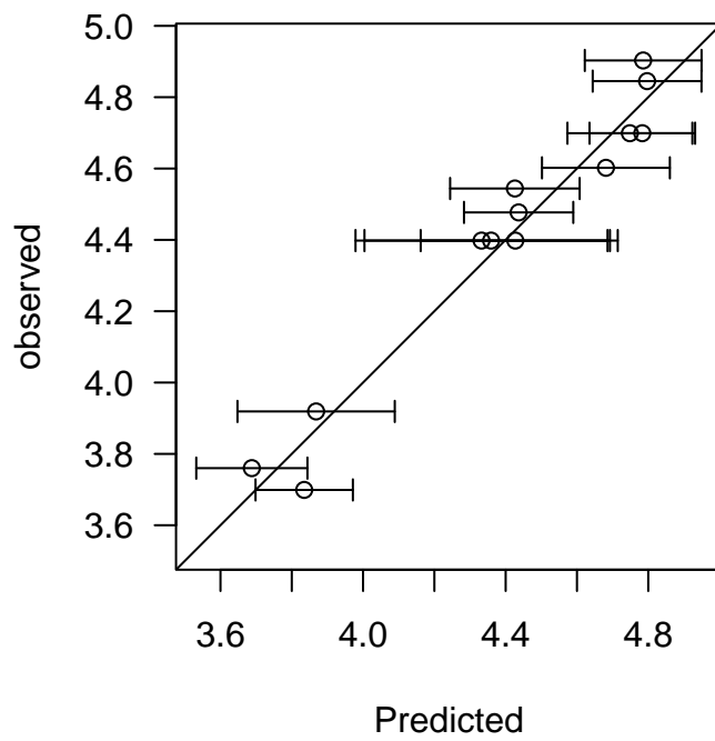
Figure 2: Predicted and observed \log_{10} neonatal body mass for 13 odd-toed ungulate species.
