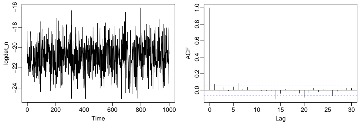
Figure 5: Trace plot and empirical autocorrelation function of the log determinant of the model-implied covariance matrix at t = n .
