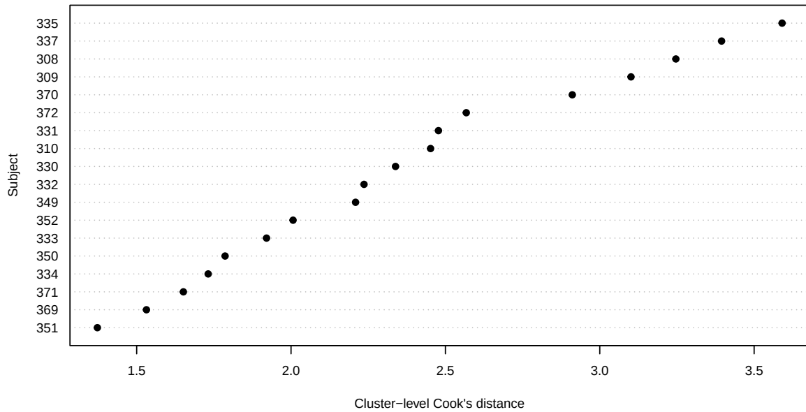
Figure 1: Per-subject (cluster-level) Cook's distances for the robust sleepstudy fit. Subjects at the top are the most influential on the joint parameter vector (\hat{\beta}, \hat{\sigma}, \hat{\theta}) .
